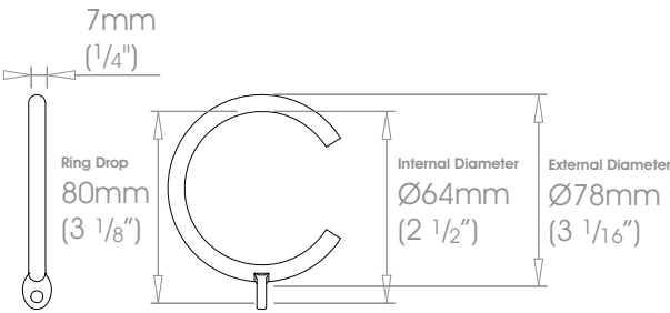
50mm (2") Passing Ring
