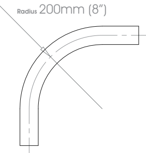
50mm (2") Brass Bay Bend
