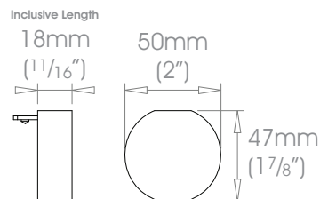
Round 50mm (2") Flush Stud
