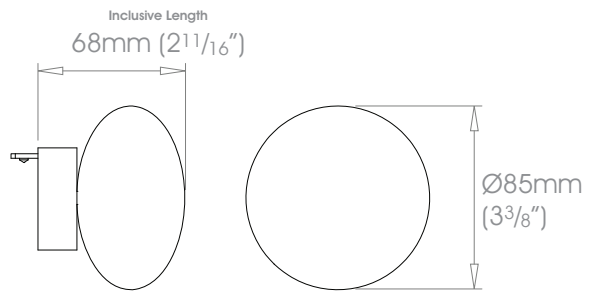
50mm (2") Pebble
