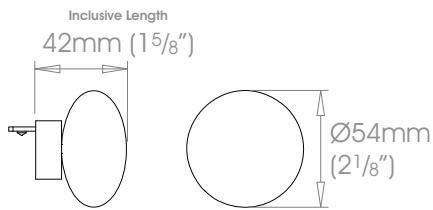
30mm (1 3/16") Pebble
