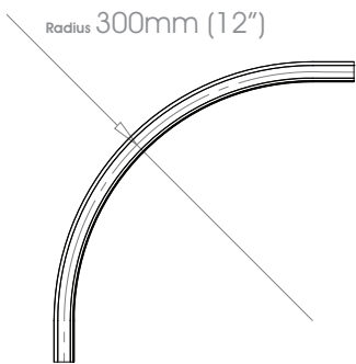
Radius 300mm (12") Square 37mm (1 1/16") Bay Bend
