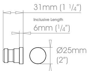
25mm (1") Flush Stud
