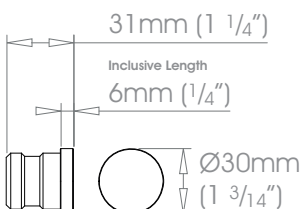
30mm (1 3/16") Flush Stud
